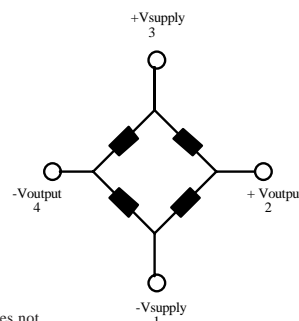
Equivalent Circuit
